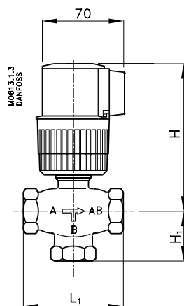
VMV + ABV
